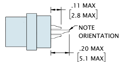
3 ROW CONNECTOR
